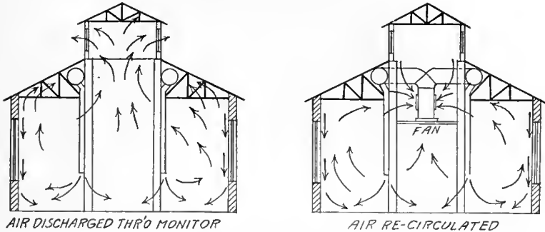
FIG. 13. TWO METHODS OF AIR DISTRIBUTION IN AN INDUSTRIAL BUILDING
